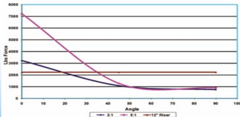
Pull Force Vs. Angle
